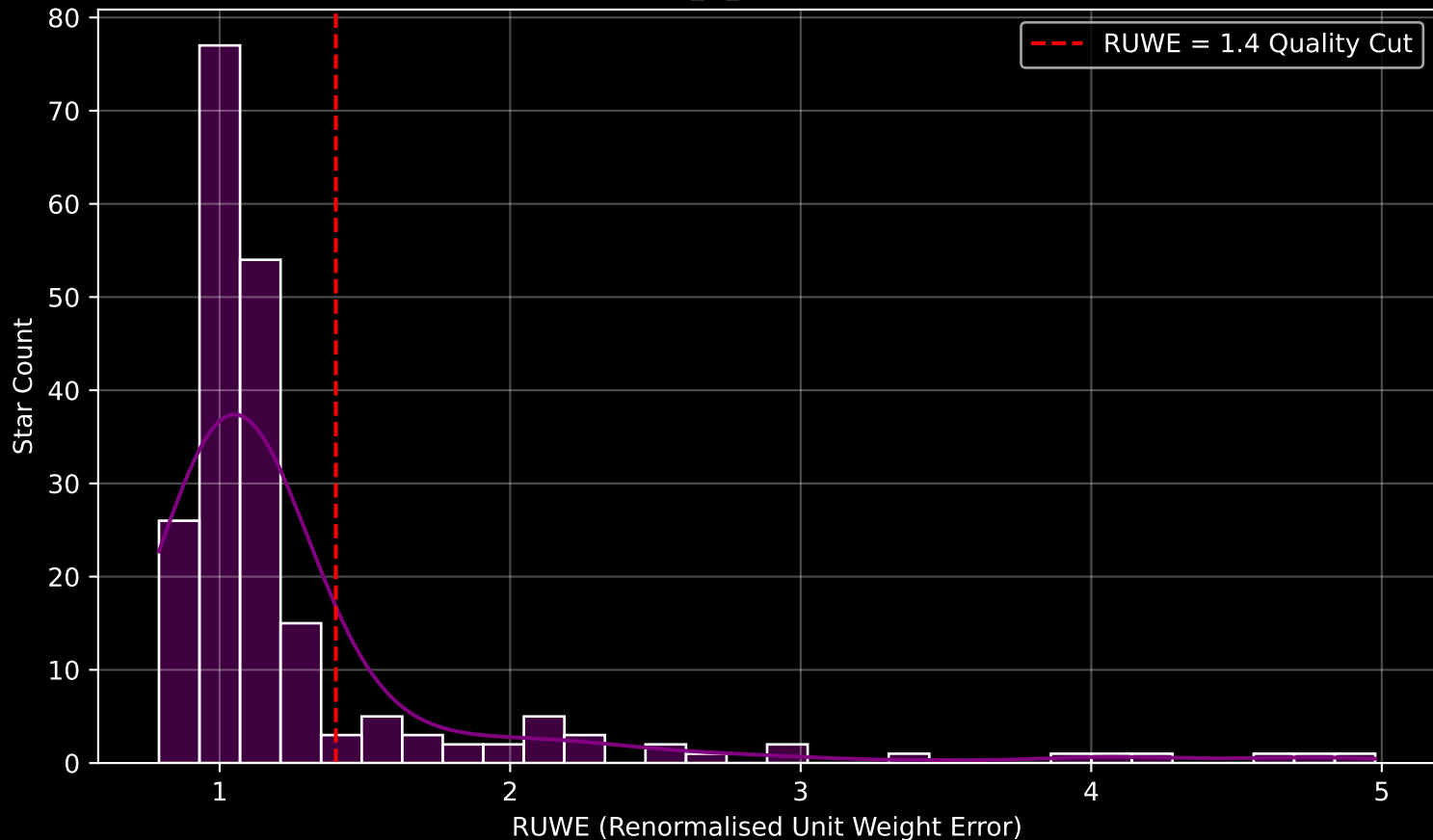
GAPOGEE DR17 Field [Cet_M_MGA] RUWE Distribution (n= 207)
