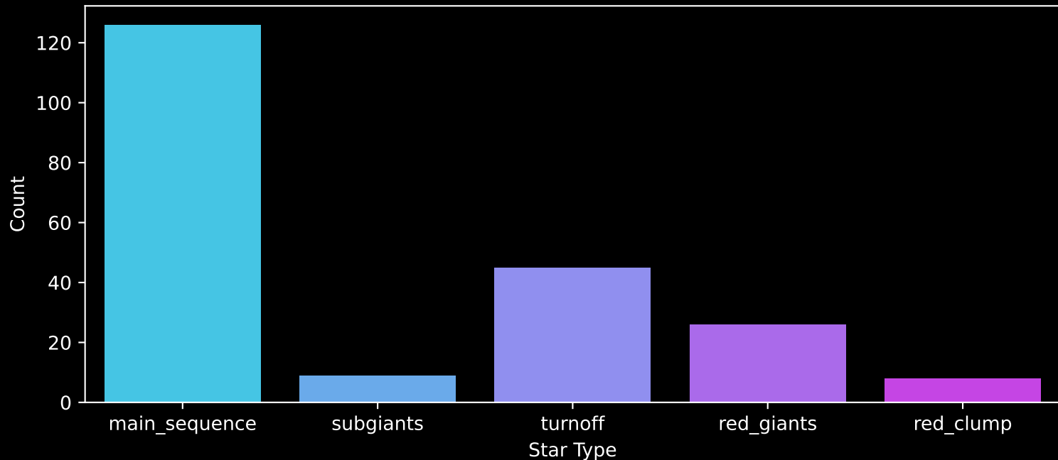
APOGEE DR17 Field: [Cet_M_MGA] Count plot of Star Type
