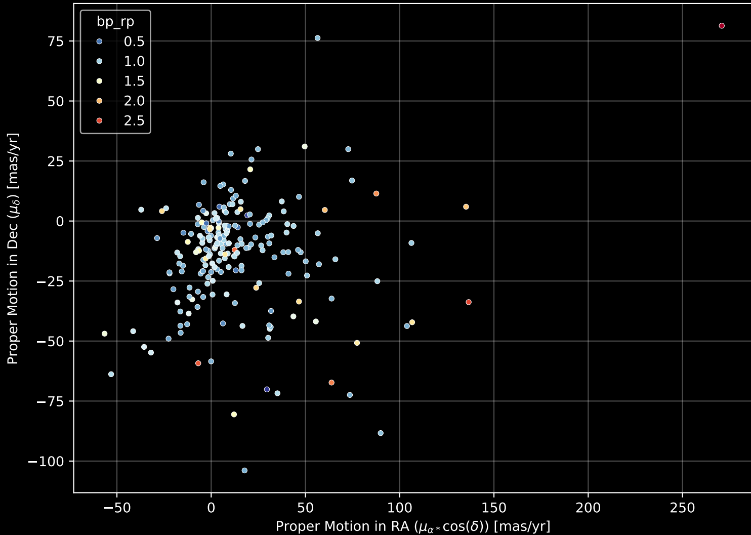
APOGEE DR17 Field: [Cet_M_MGA] Proper Motion Diagram (n= 214)
