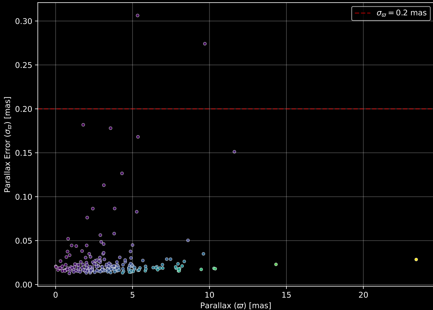
APOGEE DR17 Field: [Cet_M_MGA] Parallax Quality (n= 214)
