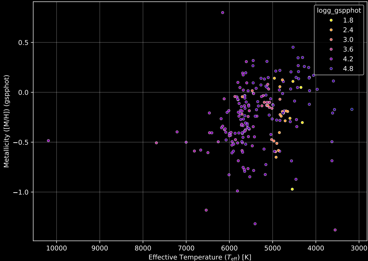
APOGEE DR17 Field: [Cet_M_MGA] Stellar Population Parameters (n= 214)
