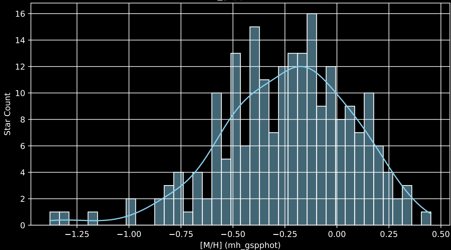
APOGEE DR17 Field: [Cet_M_MGA [M/H] (mh_gspphot) (n= 213)
