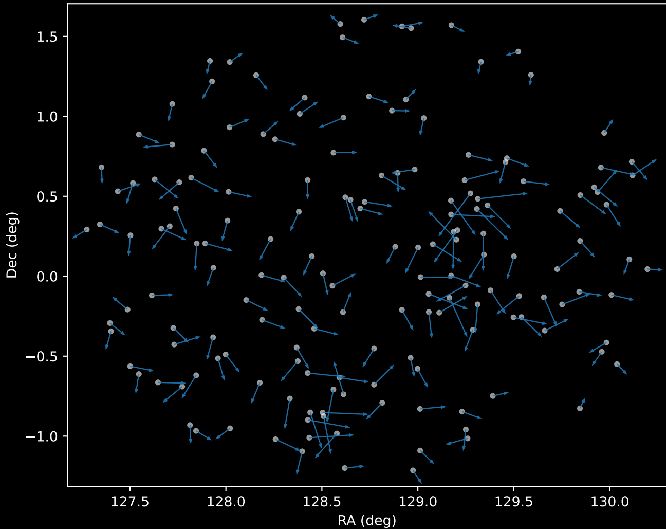
APOGEE DR17 Cluster 0 Proper Motion Vectors (n=167)
